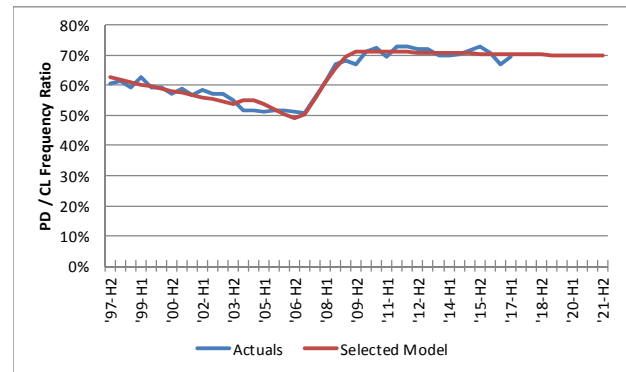
Industry Alberta PPV – ratios of select coverage frequencies (both “actual” and “modeled”; ultimates as selected by FA as at Jun 30, 2017)
